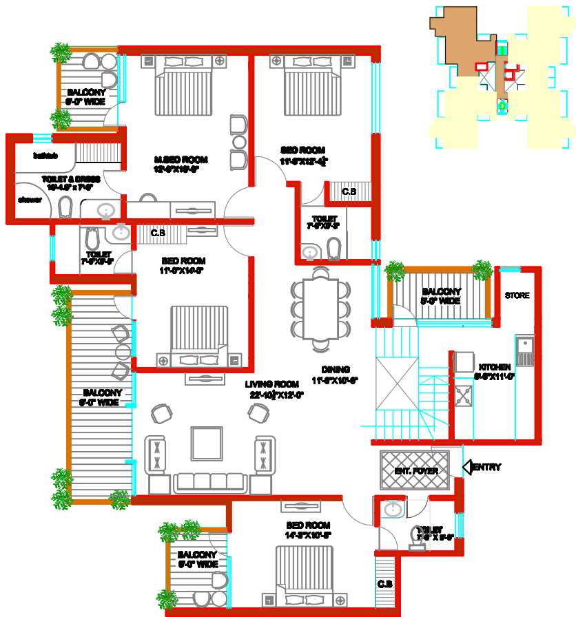
PENT HOUSE ( Lower floor ) 5 BED ROOM UNIT
